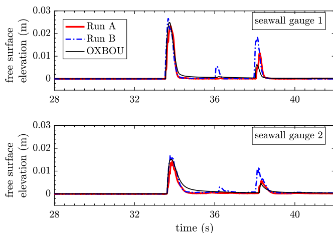
Fig. 5. Free-surface elevation time-histories by seawall gauges 1 and 2 (corresponding to wave gauges 11 and 12 in Fig. 1), located at the most seaward and central points on the seawall crest; laboratory measurements (red, blue) and OXBOU predictions (black). A = 0.0855 m, x_f = 5.0 m relative to the beach toe, \phi = 180^\circ .
