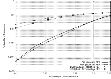
Fig. 2. Hermitian [60,45,10] vs BCH[60,45,9] in the erasure channel
