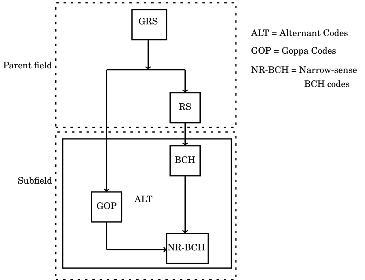
Fig. 3.1: Relationship between algebraic codes
