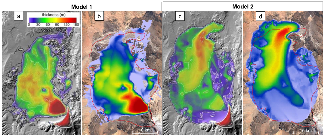
Figure 3. Final deposit thickness of the Socompa avalanche considering frictional rheological law with \phi_{bed} = 2.5^\circ and in an isotropy condition of stresses in VolcFlow code (a) and RASH3D code (b). Figures c and d show the obtained final deposit considering a constant retarding stress rheological law with \tau = 52 kPa in VolcFlow code (c) and RASH3D code (d).
