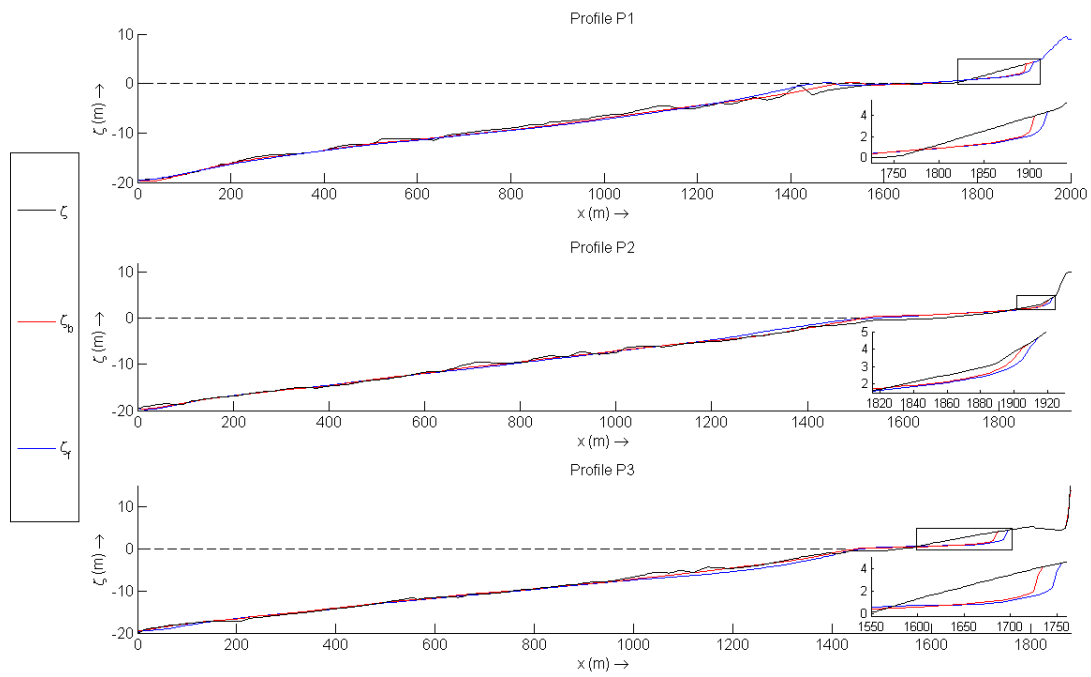
504 Figure 14: Bed level at profiles P1, P2 and P3: before the storm ( \zeta_\theta ) [07 Dec 2007, 12:00 UTC] and 505 after the storm [16 Nov 2007, 06:00 UTC] in the baseline scenario ( \zeta_b ) and with the wave farm ( \zeta_f ). 506 [Profiles P1, P2 and P3 are delimited in Figure 3].
