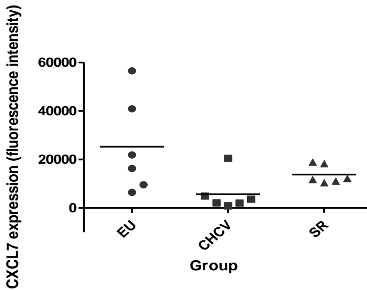
Figure 3-7 Fluorescence intensity of CXCL7 between EU, CHCV and SR.
