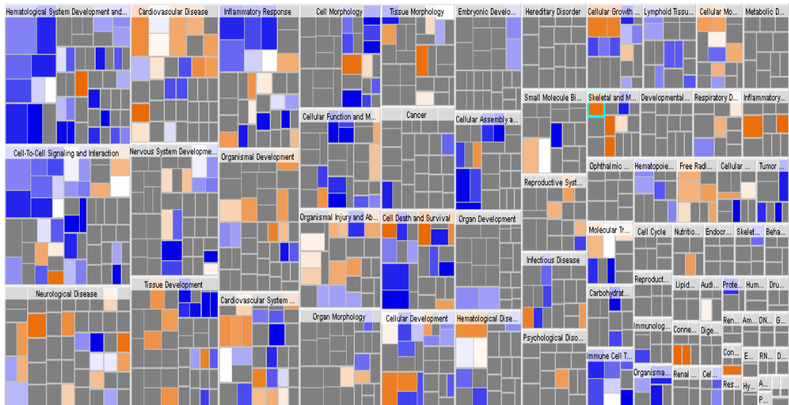
Figure 3-3 Downstream effects analysis (“heat map”) of the CHCV vs EU groups.
