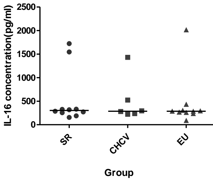
Figure 5-2 Scatterplot of IL-16 concentration in SR, CHCV and EU.
