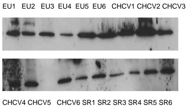
Figure 6-11 Phospho-Akt (pThr308) Western blot.
