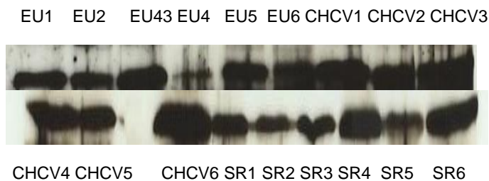
Figure 6-9 PI3K-p110δ Western blot.
