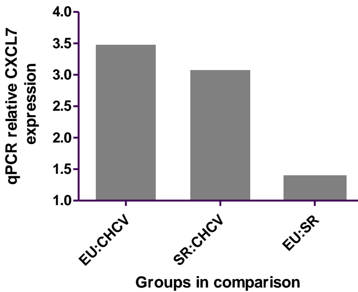
Figure 4-2 CXCL7 qPCR in comparison groups.
