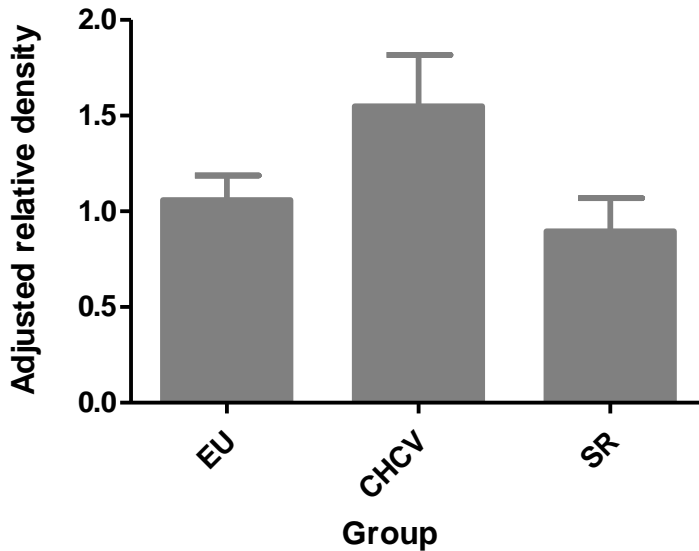
Figure 6-12 Phospho-Akt (pThr308) mean adjusted relative density between EU, CHCV and SR.
