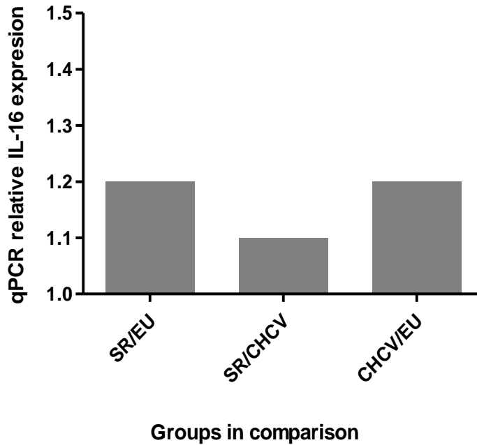
Figure 5-1 IL-16 qPCR in comparison groups.
