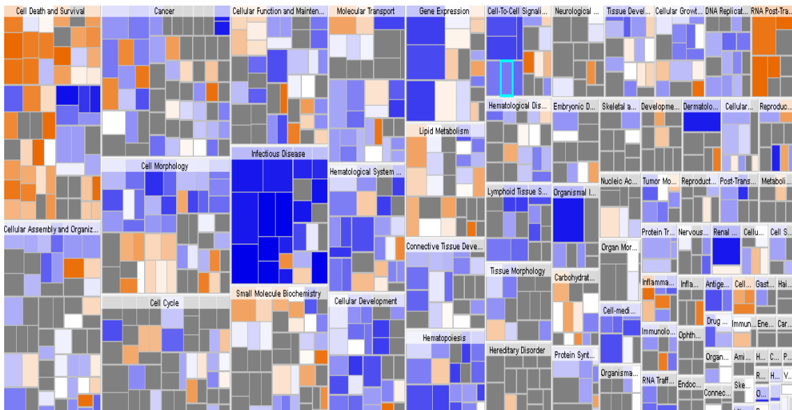
Figure 3-4 Downstream effects analysis (“heat map”) of the CHCV vs SR groups.
