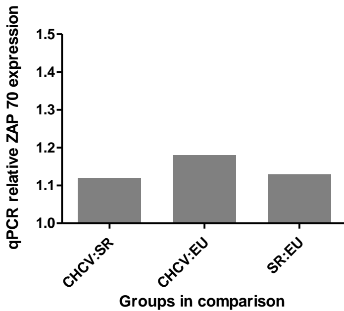
Figure 6-5 ZAP70 qPCR in comparison groups.
