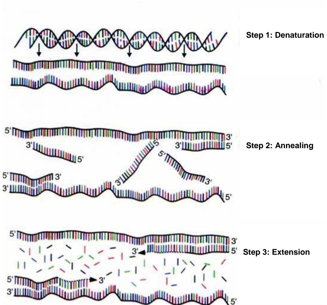
Figure 2-1 The PCR process.
