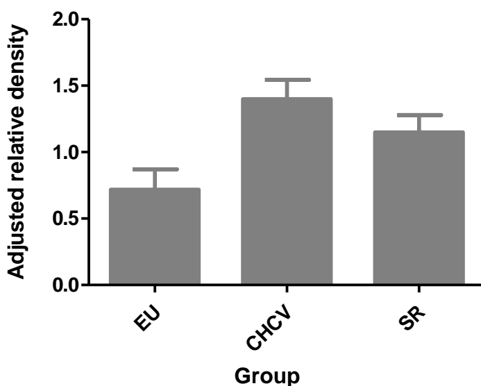
Figure 6-15 Phospho-Akt (pSer 473) mean adjusted relative density between EU, CHCV and SR.
