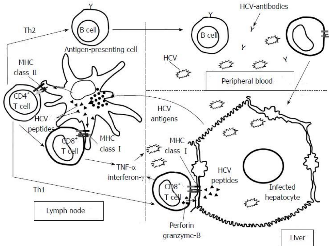
Figure 1-5 HCV specific adaptive immune response.
