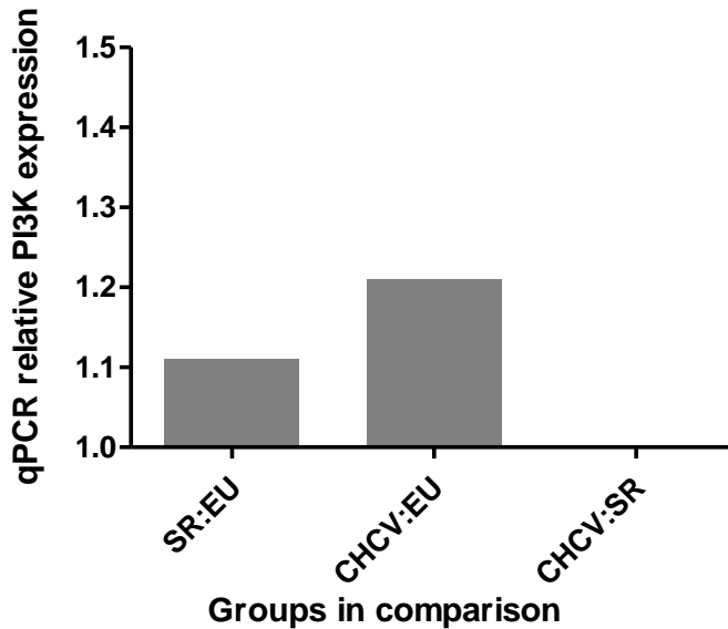
Figure 6-3 PI3K qPCR in comparison groups.
