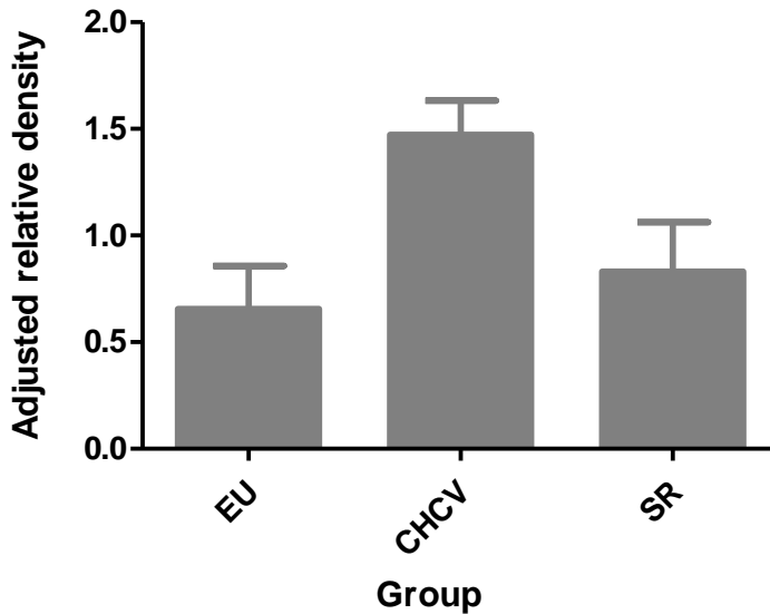
Figure 6-10 PI3K-p110δ mean adjusted relative density between EU, CHCV and SR.
