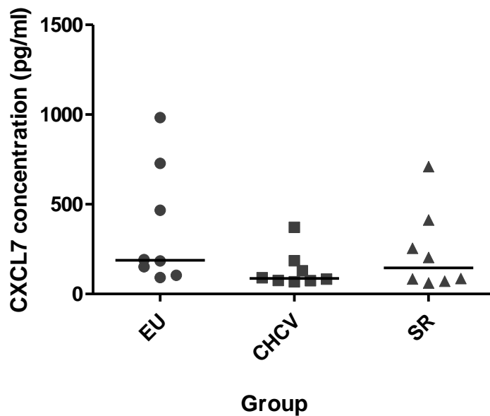
Figure 4-4 Scatterplot of CXCL7 concentration in EU, CHCV and SR.
