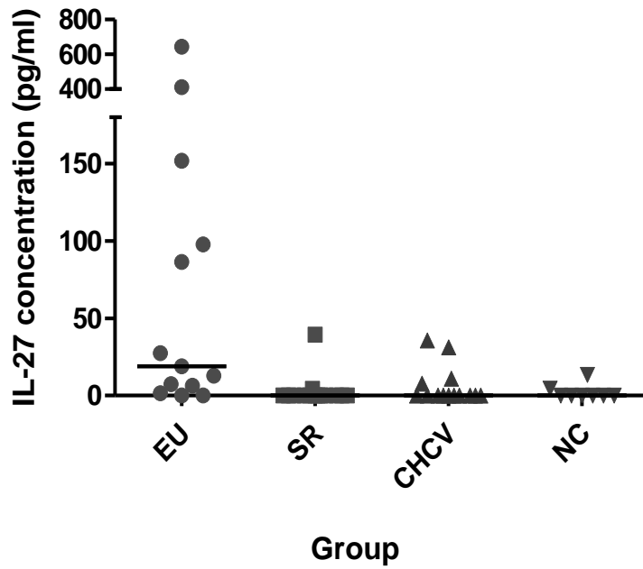
Figure 4-3 Scatterplot of IL-27 in EU, CHCV, SR and NC.
