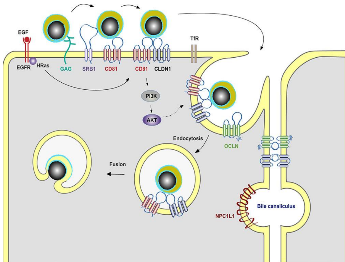
Figure 1-2 HCV entry.
