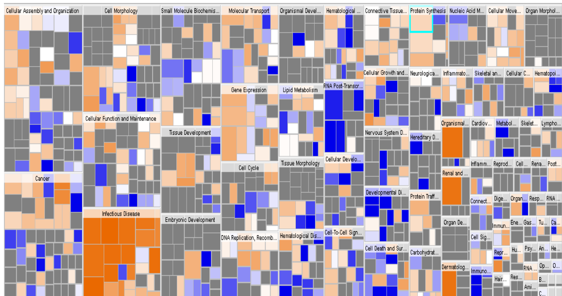
Figure 3-5 Downstream effects analysis (“heat map”) of the SR vs EU groups.
