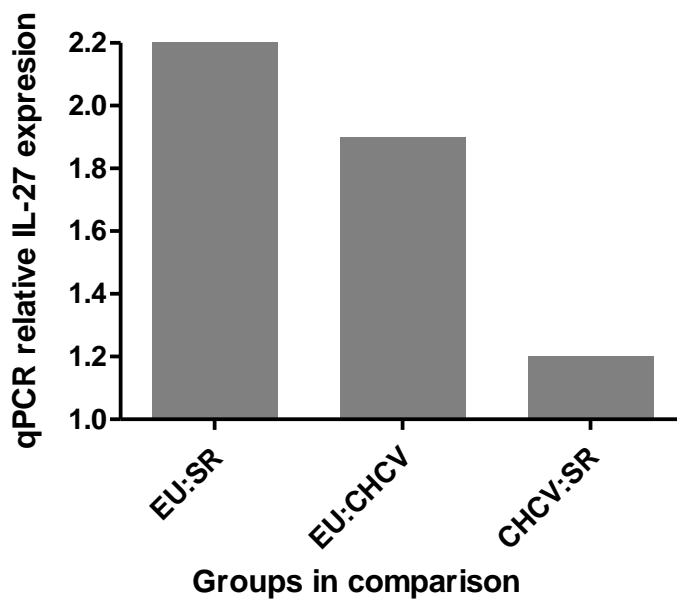
Figure 4-1 IL-27 qPCR in comparison groups.
