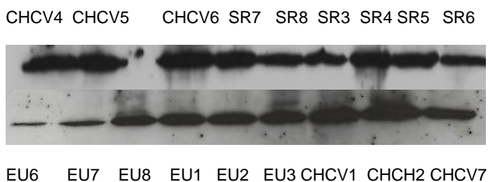
Figure 6-14 Phospho-Akt (pSer473) Western blot.
