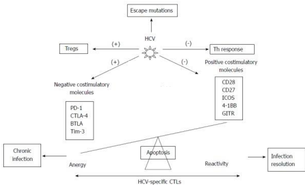
Figure 1-6 Hepatitis C virus strategies to escape from hepatitis C virus-specific cytotoxic T cells control.
