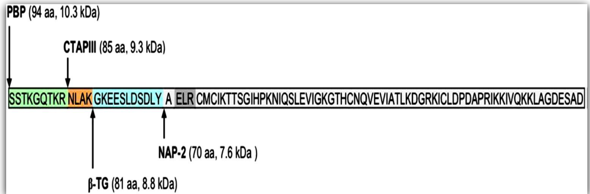
Figure 4-5 Amino acid sequences of CXCL7 derivatives.
