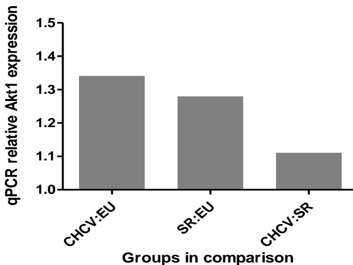
Figure 6-4 Akt1 qPCR in comparison groups.
