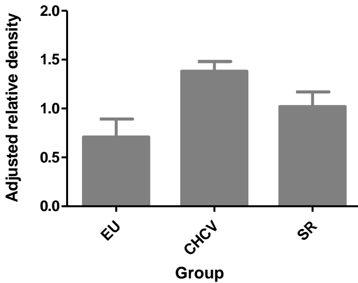
Figure 6-8 Pan-Akt adjusted mean relative density between EU, CHCV and SR.
