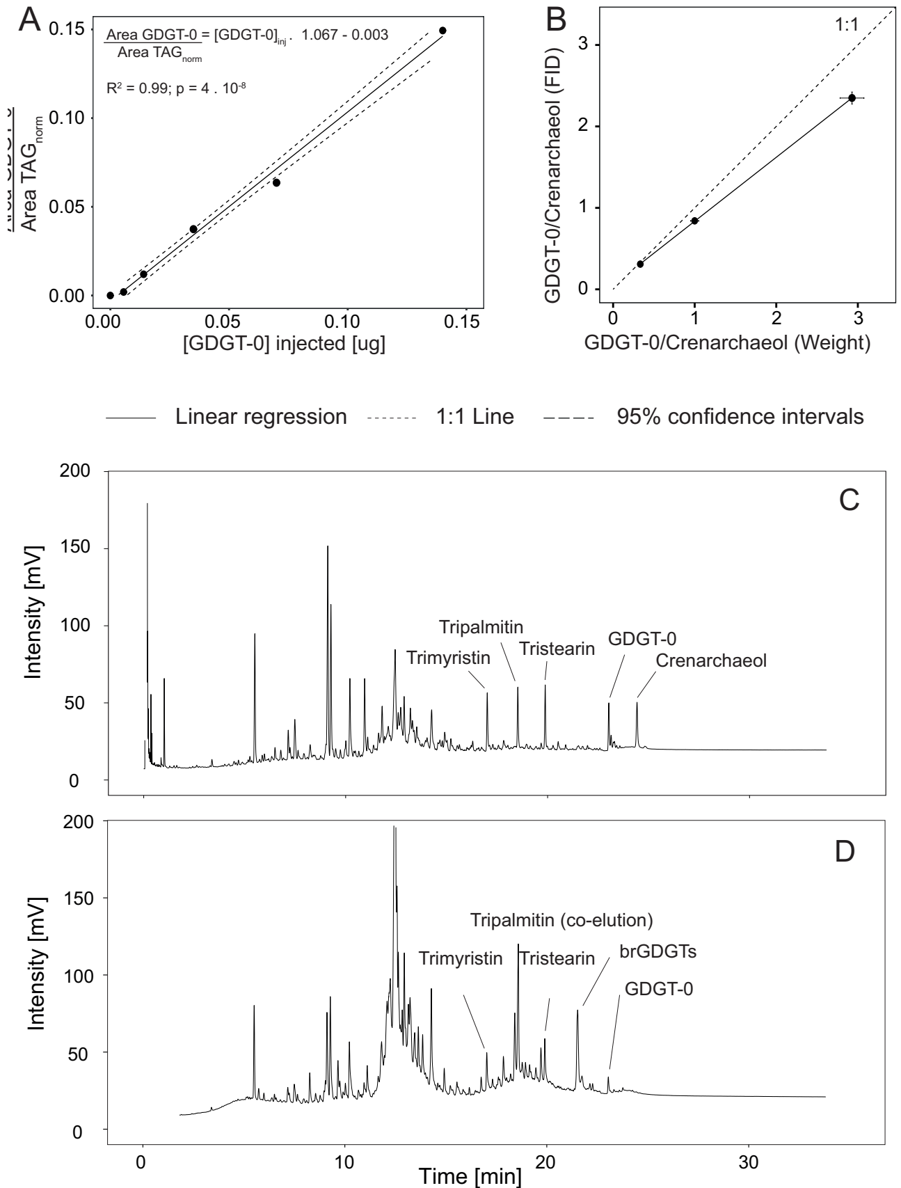
Figure 4. Quantification of GDGT-0. A) Correlation of Peak area ratios GDGT-0/trimyristin (normalised on µg trimyristin injected) with the amount of GDGT-0 injected in µg; B) Crenarchaeol/GDGT-0 peak area ratios determined from three mixtures of purified compounds of different relative composition (GDGT-0/Crenarchaeol = 1:1, 1:3.1, and 4:1.2); C and D show chromatograms of the peat and marine standards with added TAG standards.
