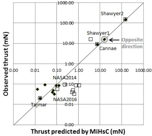
Figure 2. A comparison between the eleven observed emdrive thrusts (on the y axis) and the thrusts predicted by quantised inertia (on the x axis) without considering the effect of dielectrics (the empty squares) and considering the effect of the dielectrics (the black diamonds). When the dielectrics were considered the results were far better (closer to the diagonal line), except for Shawyer1 where the prediction was the right size but in the wrong direction.
