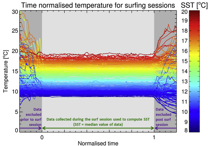
Fig. A3. A superposition of all temperature data acquired by the surfer during the study period, normalised such that the start (0) and end (1) of the surfs are at the same point on the x-axis for each session. Data in dark grey were excluded and light grey included. The data in light grey were used to compute SST by taking the median of this data.
