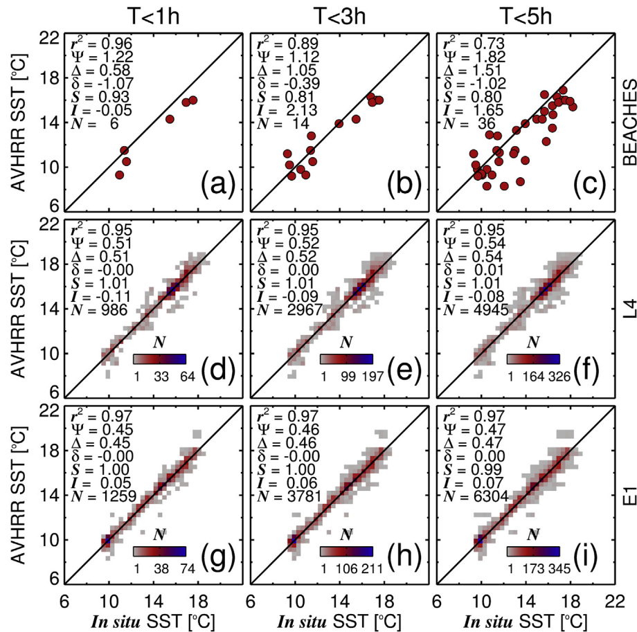
Fig. 7. Scatter plots of Level 3 AVHRR satellite passes and in situ sea surface temperature (SST) data for an absolute time difference ( T ) of <1\text{h} , <3\text{h} and <5\text{h} , at the coastline (a–c), at L4 (d–f) and at E1 (g–i). r^2 is the coefficient of determination, \Psi the root mean square error, \delta the bias, \Delta the centre-pattern (or unbiased) root mean square error, S the slope and I the intercept of a linear regression, and N the number of samples.
