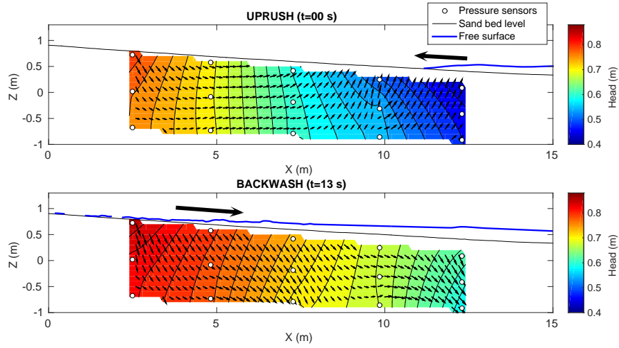
Figure 8: Groundwater pressure head and velocity fields during uprush (top plot) and backwash (bottom plot) phases of an IG-driven swash event measured during the Rousty1412 field campaign in the Rousty beach (Camargue, France). The blue solid line indicates the free surface elevation measured by terrestrial LiDAR while the solid black line indicates the sand bed. Each white circle within the sand soil corresponds to a buried pressure sensor (5Hz acquisition frequency). Color contours indicate the groundwater head field, interpolated from measurements at each sensor. Vectors are groundwater velocities calculated from the head field using the Darcy's law.
