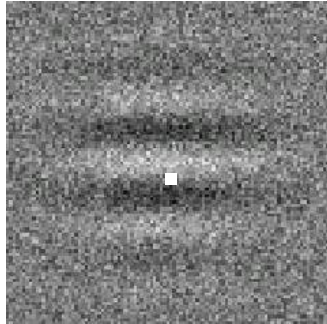
Figure 1. Illustration of a single frame of the 2 c/deg grating stimulus with added noise. On each trial, the observer fixated a central point and reported whether the stimulus contained a moving grating or a blank field (detection task); a counterphase flickering grating or a blank field (summation task) or an upwards or downwards moving grating (discrimination task) in different levels of added noise.
