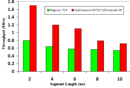
Fig. 7. The impact of segment length on throughput
