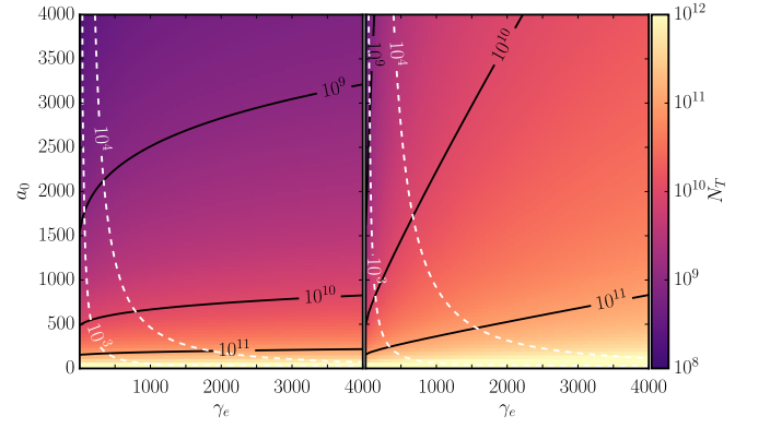
FIG. 1. The number N_T of radiating electrons required to see significant depletion plotted as a function of \gamma_e and a_0 . Black curves indicate the depletion thresholds a_0(\gamma_e) when N_T = 10^9 , 10^{10} and 10^{11} . The dashed white curves represent \omega' \Delta x = \text{const} \gg 1 , so that photon emission is incoherent across the relevant parameter space. Left: using (4). Right: using (6) below.
