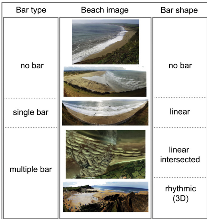
Fig. 5. Classification of bar type and shape with associated examples from remote image dataset.
