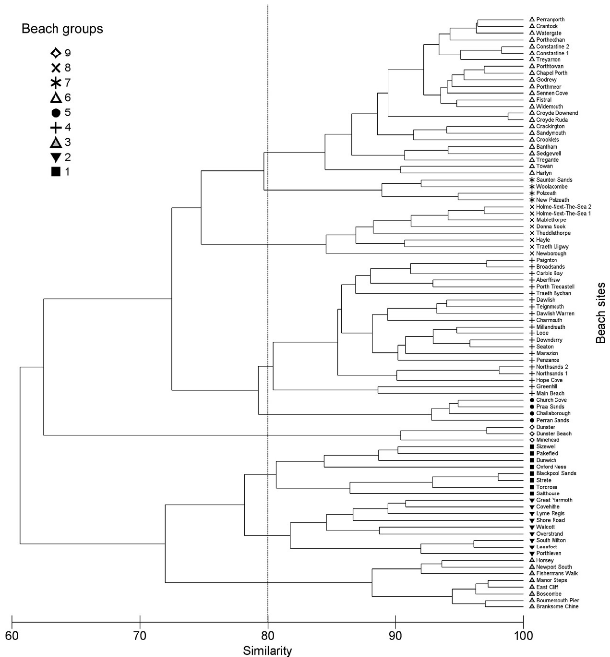
Fig. 9. Dendrogram clustered using unweighted pair group average (UPGMA) method. Symbols represent discrete beach groups attained using a cut-off level of 80% similarity. Numbering is arbitrary and represents a coarse reflective to dissipative order to aid further interpretation.
