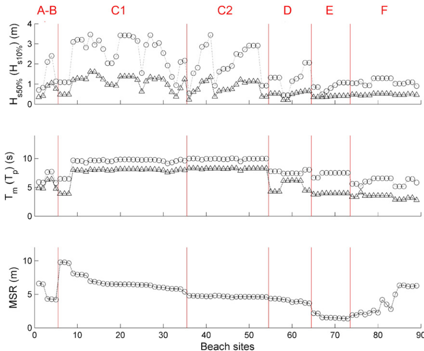
Fig. 6. Inshore hydrodynamic conditions for each beach site moving anti-clockwise around the coast: (top) 50% exceedance significant wave height (triangles) and 10% exceedance significant wave height (circles); (middle) mean wave period (triangles) and peak wave period (circles); and (bottom) mean spring tidal range. A Liverpool Bay; B Irish Sea; C1 Atlantic southwest (north coast); C2 Atlantic southwest (south coast); Lyme Bay; Channel Coast; East Coast.
