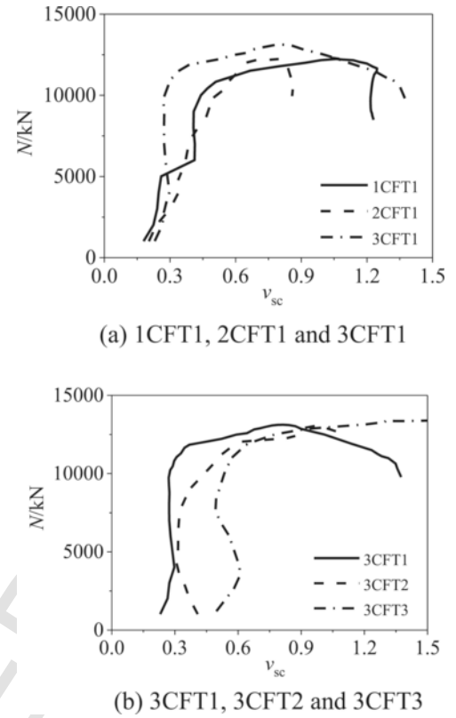
Fig. 8. Axial load vs. Poisson's ratio curves of the steel tubes among 1CFT, 2CFT and 3CFT.
