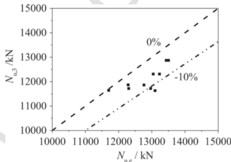
(a) Comparison of ultimate bearing capacities obtained from Eq. (17) and test results
