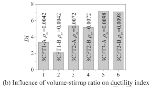
Fig. 7. Comparison of ductility indexes for all specimens.
