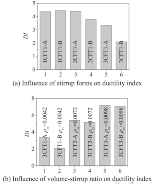
Fig. 7. Comparison of ductility indexes for all specimens.
