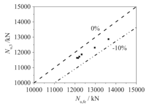
(b) Comparison of ultimate bearing capacities obtained from Eq. (17) and FE results
