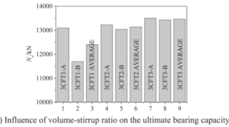
Fig. 6. Comparison of ultimate bearing capacities for all specimens.
