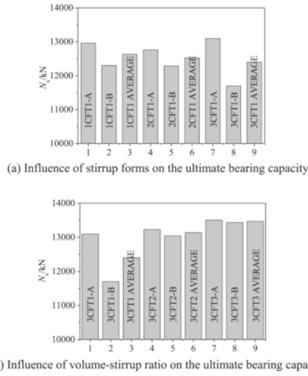
Fig. 6. Comparison of ultimate bearing capacities for all specimens.
