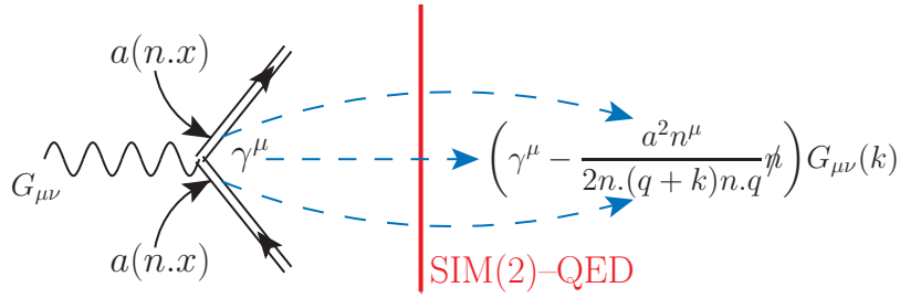
FIG. 2. Products of background field propagators (double lines, left) across vertices in QED generate slowly varying terms necessary to preserve the Ward-Takahashi identity, and generate the three-point SIM(2)-vertex (right).
