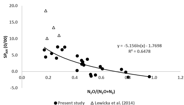
Figure 3. Ratio \text{N}_2\text{O} / (\text{N}_2\text{O} + \text{N}_2) vs. site preference (SP) for all for treatments in the first 2 days. A logarithmic function was fitted through the data; the corresponding equation and correlation coefficient are given. Also shown data from Lewicka et al. (2014).
