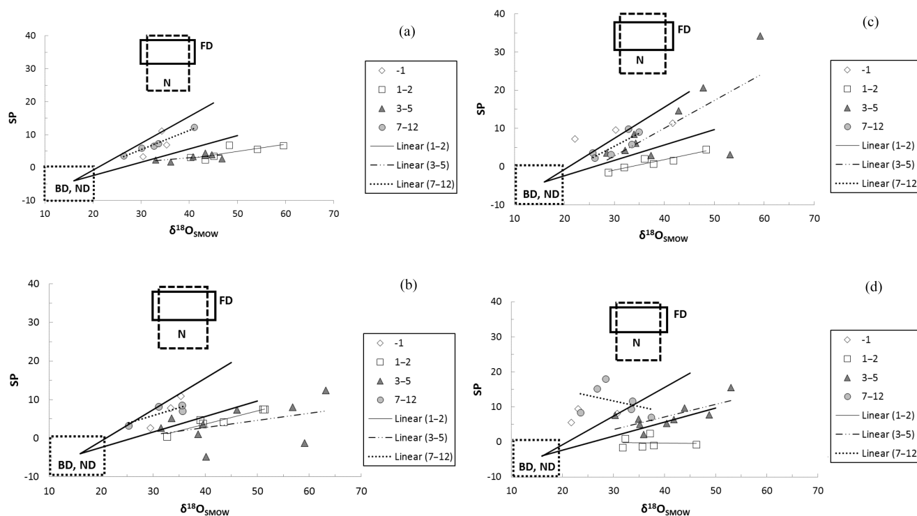
Figure 5. Site preference (‰) vs. \delta^{18}\text{O} (‰) in all treatments for three periods (day –1, days 1–2 and days 3–12) in the experiment: (a) SAT/sat treatment; (b) HALFSAT/sat; (c) UNSAT/sat; (d) UNSAT/halfsat. Equations of fitted functions and correlation coefficients are in Table 7 for 1–2, 3–5 and 7–12 (5–12 for c). Endmember areas for nitrification, N; bacterial denitrification, D; fungal denitrification, FD; and nitrifier denitrification, ND, as well as corresponding vectors or reduction lines (black solid lines) are from Lewicka-Szczepak et al. (2017) and represent minimum and maximum routes of isotopocule values with increasing \text{N}_2\text{O} reduction to \text{N}_2 based on the reported range in the ratio between the isotope fractionation factors of NO reduction for SP and \delta^{18}\text{O} (Lewicka-Szczepak et al., 2017).
