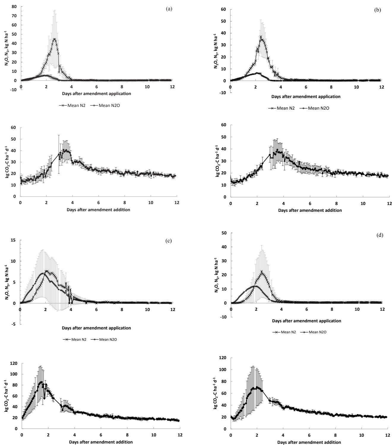
Figure 1. Mean of the three replicates for \text{N}_2\text{O} , \text{N}_2 and \text{CO}_2 emissions from (a) SAT/sat treatment, (b) HALFSAT/sat, (c) UNSAT/sat and (d) UNSAT/halfsat. Grey lines correspond to the standard error of the means (in c and d only errors for the \text{N}_2 are shown to avoid overlapping of bars).
