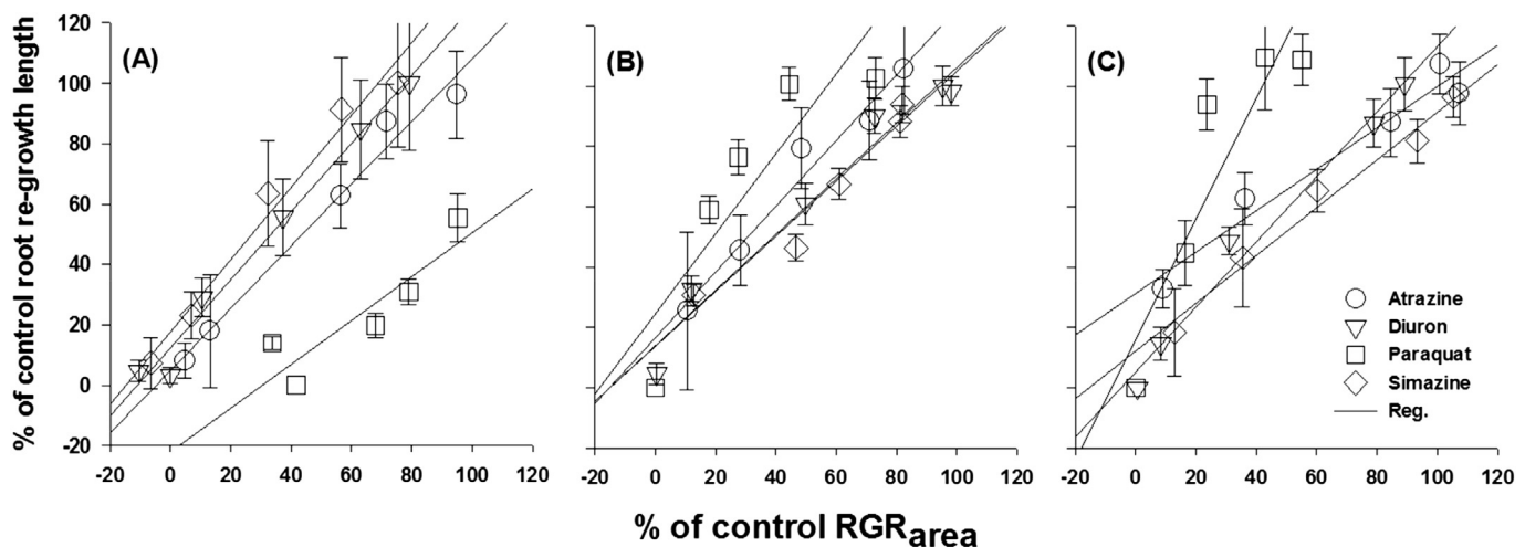
Fig. 3. Relationship between RGR_{area} and root re-growth length responses to herbicides after 72 h exposure. (A) Lemna gibba , (B) Lemna minor , and (C) Lemna paucicostata .
