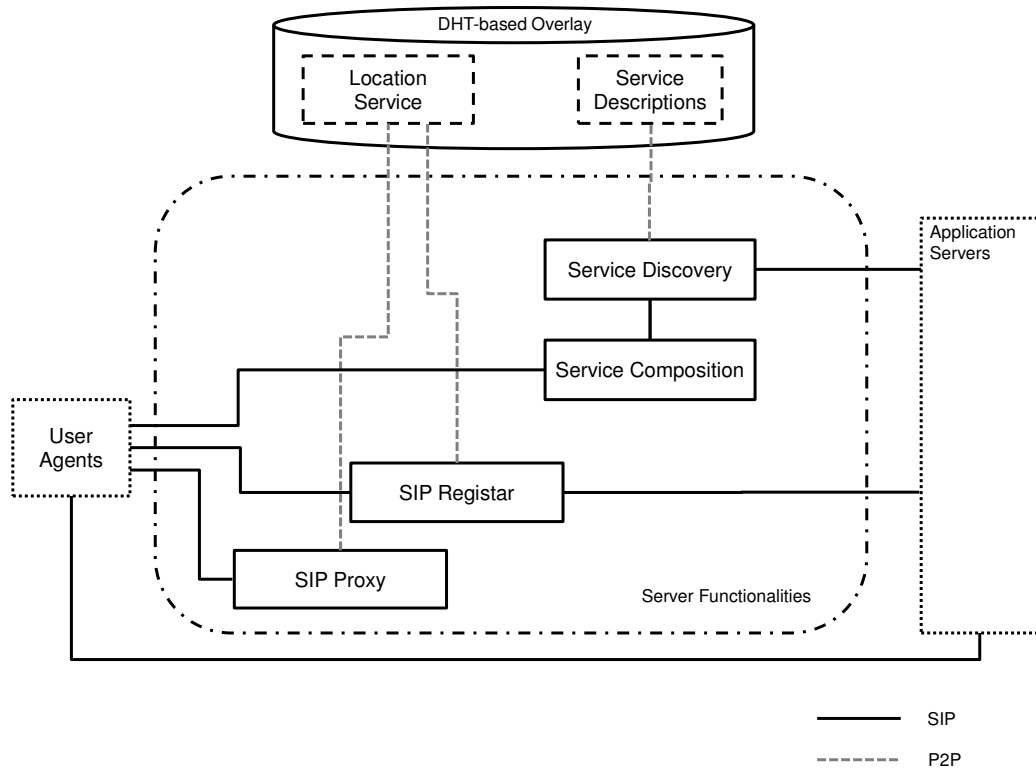
Figure 4.4: Functional framework architecture
