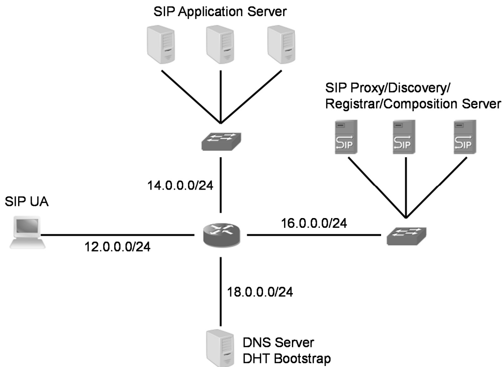
Figure 7.1: Prototype architecture
