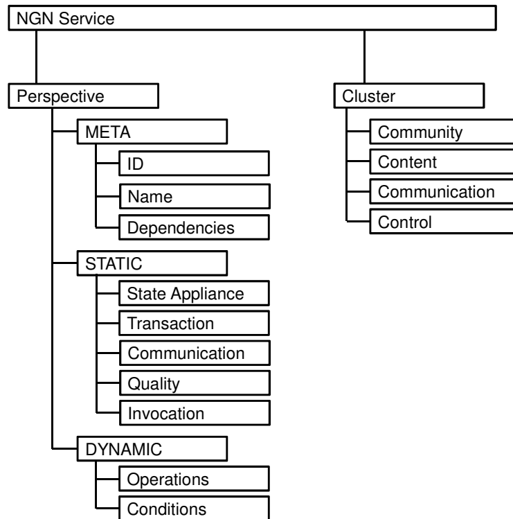
Figure 5.6: Telecommunication service ontology in (Bether, 2008)
