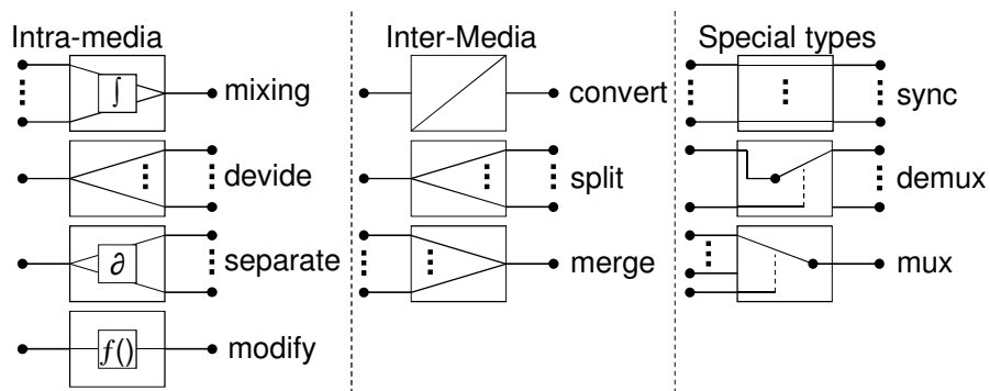
Figure 5.13: Filter types
