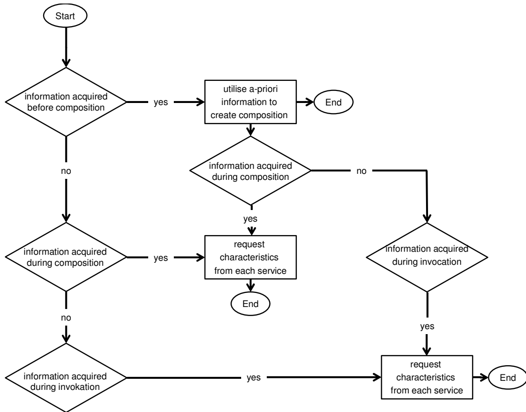
Figure 6.5: Formal notation of presented on-line techniques to reduce service interactions
