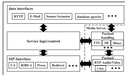
Figure 1: Application and Media Server
