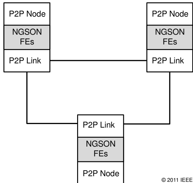
Figure 3.10: NGSON self-organized in P2P (IEEE Std 1903-2011, 2011)
