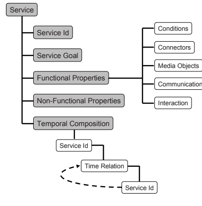
Figure 12. Structure of the Service Description Language
