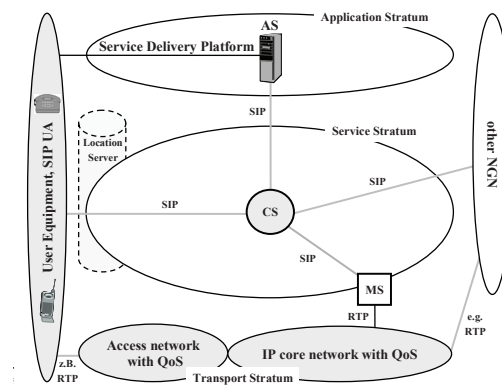
Figure 6: NGN architecture as a strata-structure
