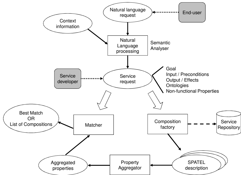
Figure 5.1: SPICE ACE architecture (Silva et al. , 2007)
