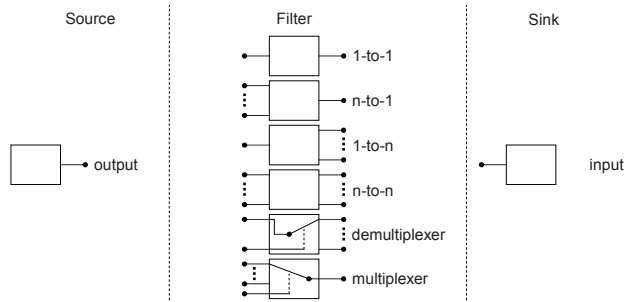
Figure 5: Basic types of media objects
