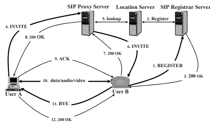
Figure 4: SIP-based client-to-client communication
