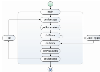
Figure 5. Wake-up Service Example
