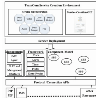
Figure 1. TeamCom Architecture
