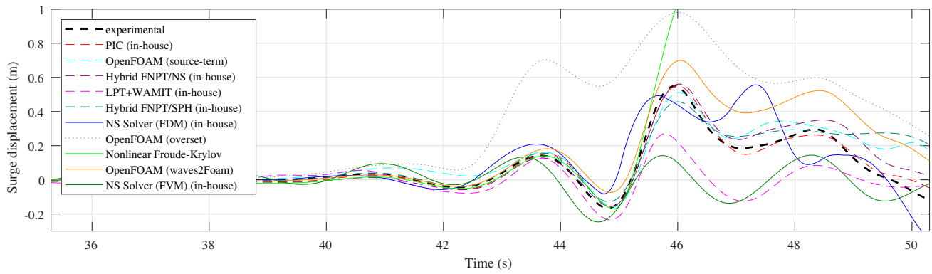
Fig. 6 Surge displacement of Geometry 1's CoM when subject to the mid-steepness wave, 2BT3. Physical measurements are plotted using a black dotted line; numerical submissions, from all participants, are shown using coloured lines.
