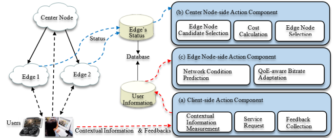
Fig. 19: An overview of QoE-aware control plane for adaptive streaming service in MEC.
