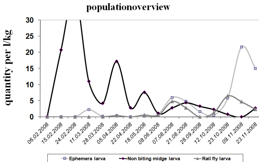
Fig. 6. Population overview
