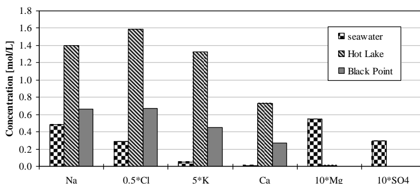
Fig. 4. End-member composition of the Hot Lake and Black Point fluids in comparison to seawater.
