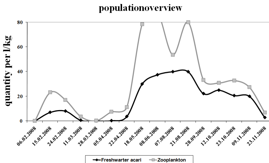
Fig. 7. Population overview
