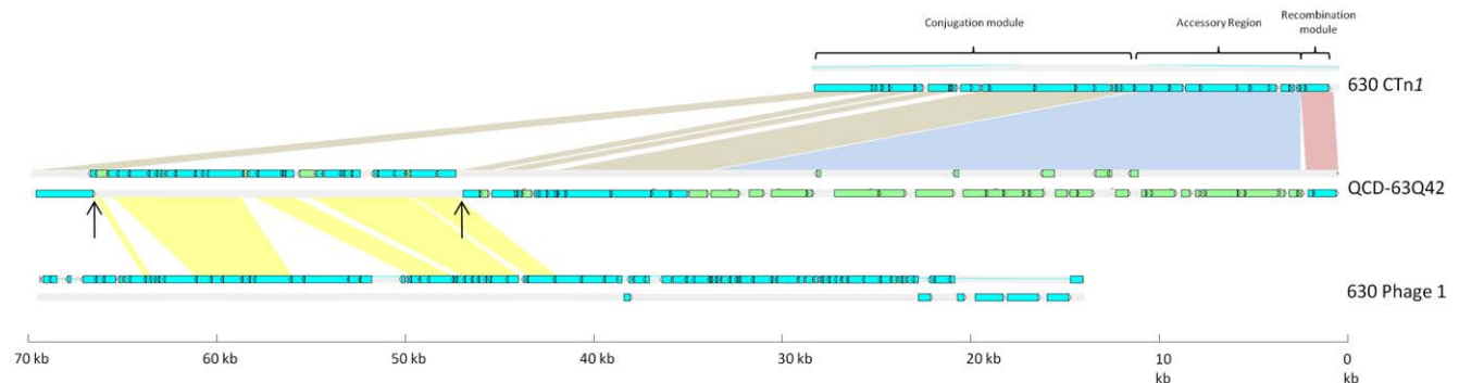
Figure 7. Schematic representation of the CTnI-like element in C. difficile QCD-63Q42. Blue ORFs have homologues present in CTnI in strain 630, green ORFs are not present in CTnI. Coloured boxes show regions of homology: red boxes show recombination modules, blue boxes show accessory genes, brown boxes show conjugation modules, yellow boxes show homologues that are not present in CTnI in strain 630. Comparison of CTnI in 630, CTnI-like element in QCD-63Q42 and phase 1 of 630. Black arrows indicate gaps in the DNA sequence. doi:10.1371/journal.pone.0023014.g007
