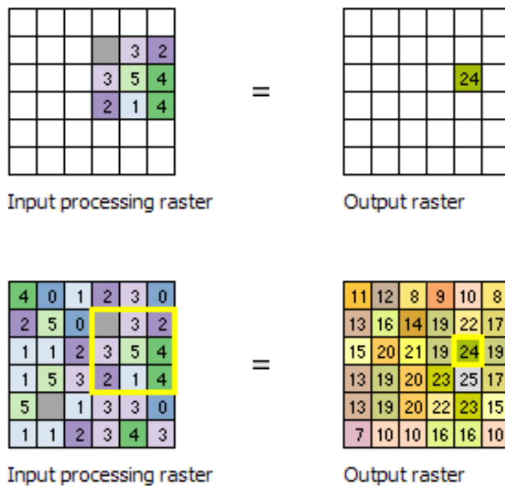
figure 4.2 Schematic for the application of focal statistics for raster (DTM) cell (ESRI, 2022).
