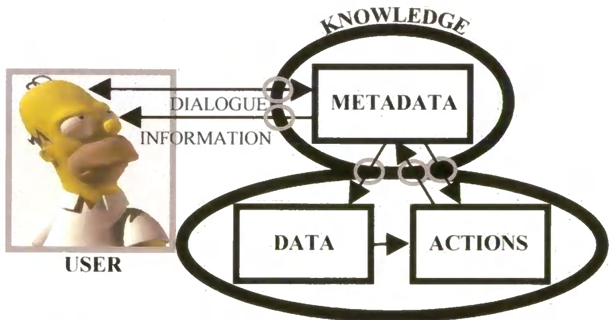
Figure 3.9: The current interplay of knowledge, information (metadata) and data in COAMES. The grey circles emphasize the role of knowledge in the system (ideally there would be use of knowledge between data and the actions applied to that data).
