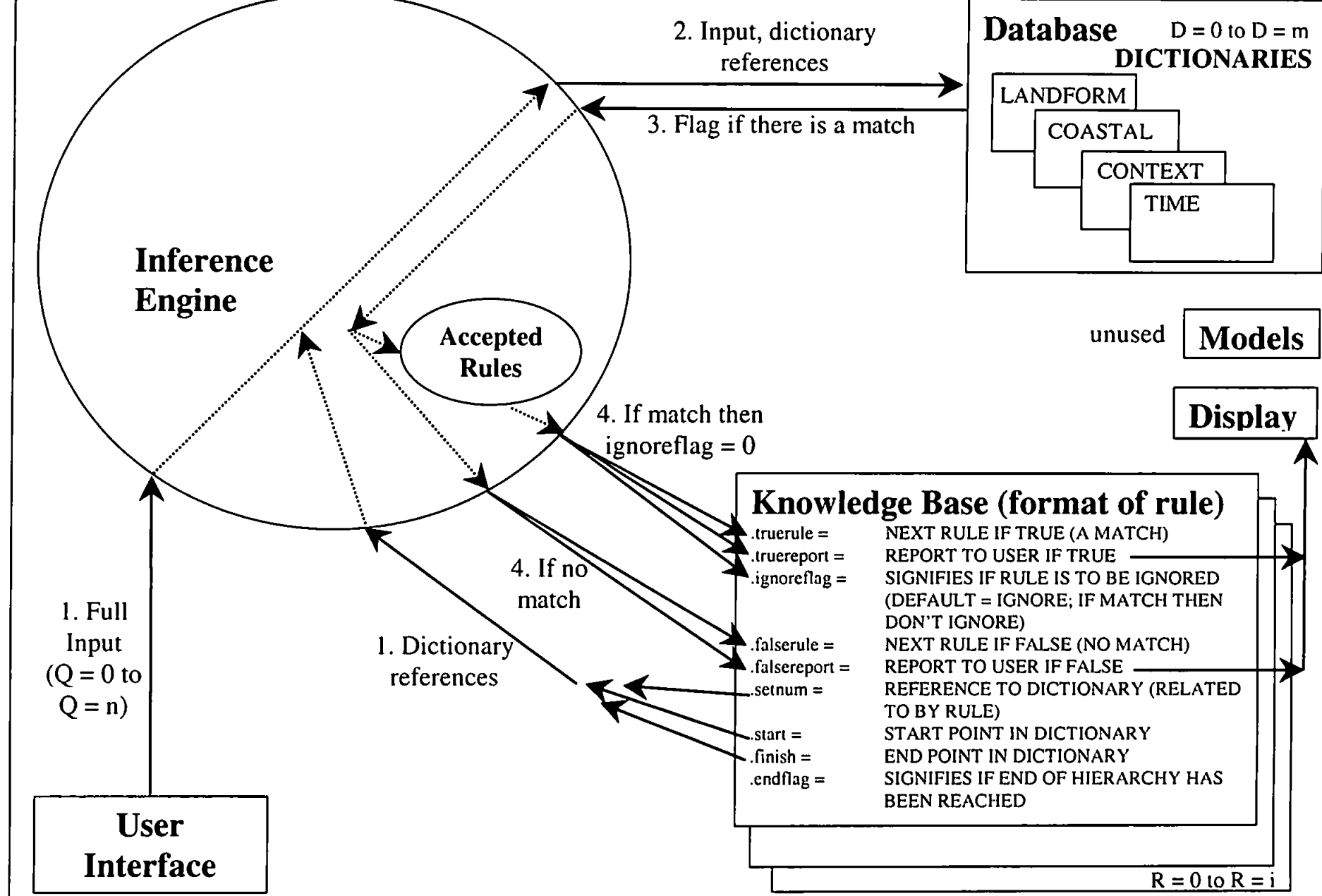
Figure 3.17: A schematic of the first stage of inference - processing the user input. {Q = a word in the input; n = number of words in the input; D = dictionary; m = number of dictionaries; R = a rule in the knowledge base; i = number of rules in the knowledge base}
