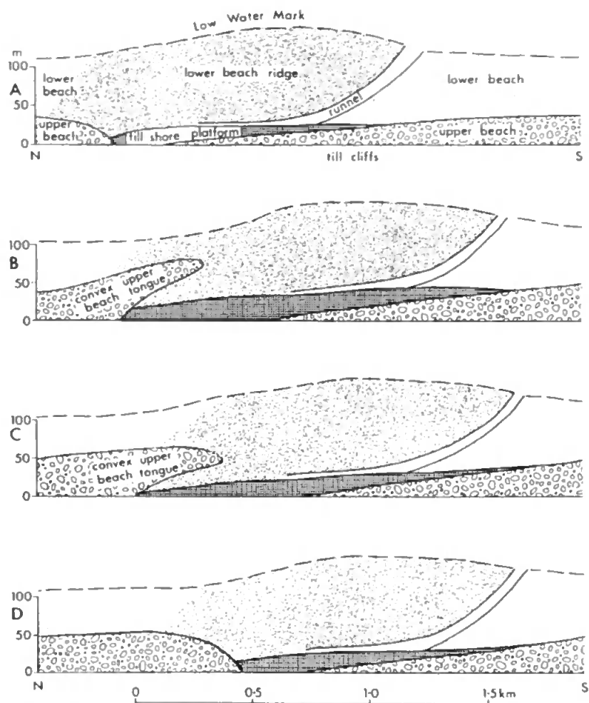
Figure 4.4: Stages in ord movement (from Pringle 1981). The initial tongue of upper beach migrates landward, whilst to the south of the section, upper beach removal leaves the till platform exposed at the foot of the cliff, moving the centre of the ord southwards.
